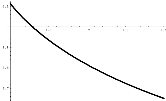
FIG. 1. Plot of the median \tilde{\mu}_\theta of f(x; \theta) as a function of \theta ( \tilde{\mu}_1 = e^{\sqrt{2}} ).
