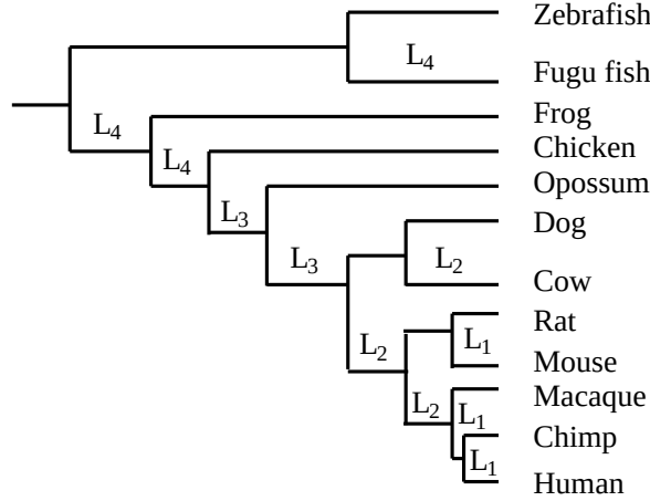
FIG. 5. Phylogenetic tree of 12 species.
