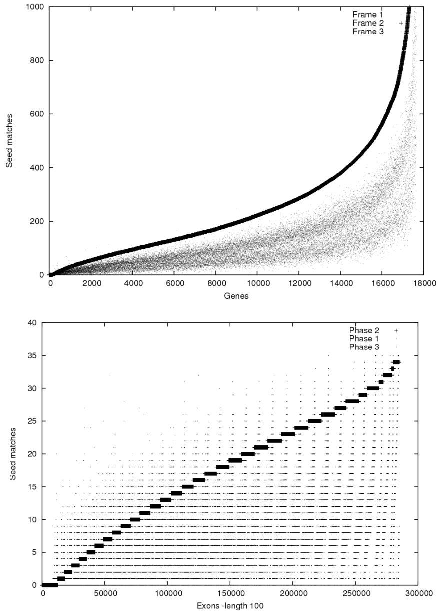
FIG. 6. Gene detection with seeds: differential frame analysis of alignments of full-length (top) and exon-size (bottom) coding regions. The numbers of seed matches in all three frames are plotted for 17,670 alignments of human and mouse gene sequences, sorted increasingly by frame 2. The test seed matches preferentially in frame 2 (thick line).
