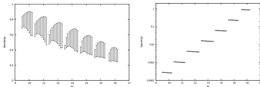
FIG. 3. Sensitivity (left, linear-scale) and specificity (right, log-scale) ranges for seeds of weight W = 10 \dots 16 , using an order 3 Markov model alignment representation for sensitivity evaluation, and using an order 1 genome Markov model and an order 2 Markov model for coding sequences for specificity. For each weight W , (n_1, n_0, n_x) combinations are shown right-to-left starting with n_x = 0 and subsequently increasing n_x . Reproduced from [24] with permission from Mary Ann Liebert, Inc.
