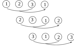
FIG. 2. Position dependencies for an order 3 inhomogeneous, 3-periodic Markov model.
