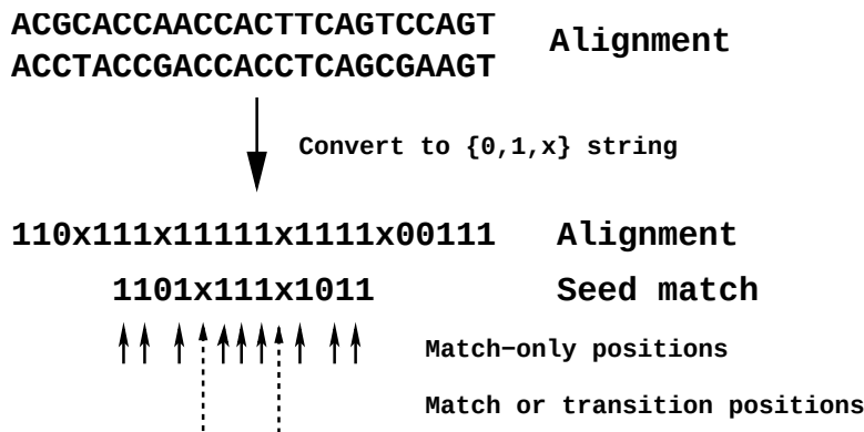
FIG. 1. Seed detection of an alignment.
