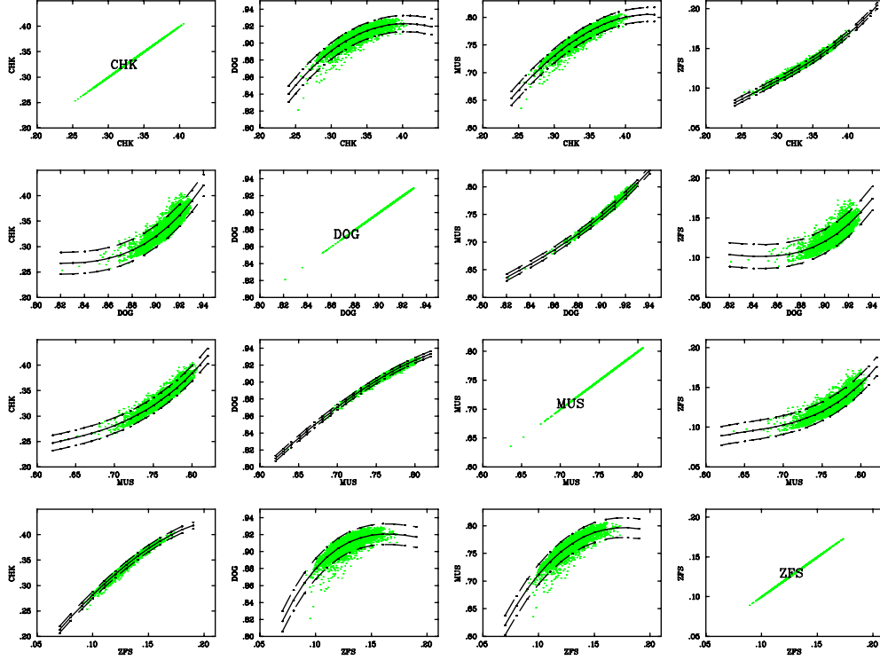
FIG. 4. Scatterplots of seed sensitivity values for pairs of comparisons among (DOG, MUS, CHK, ZFS). The non-linear regression (solid) and the 95% confidence interval (dashed) curves are shown.
